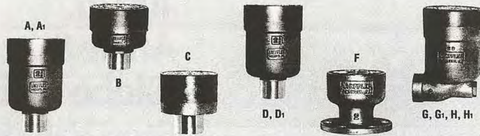
BRONZE DECK DRAINS TO NAVSEA DWG. NO. 810-1385789
