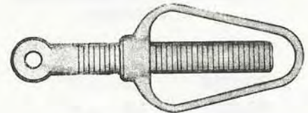
PORTLIGHT DOG Materials: Manganese Bronze Acme Threads PART # SIZE DG-1110 5/8" X 5 3/4" DG-1120 3/4" X 5 3/4"
