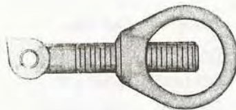
PORTLIGHT DOG Material: Manganese Bronze Acme Threads PART # SIZE DG-1130 5/8" X 4 1/2" DG-1140 3/4" X 4 1/2"
