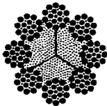
8 x 21 filler wire Type U 8 Strands, 21 Wires per Strand, 1/2 in. and larger
