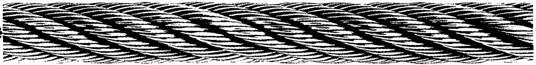
8 x 19 Warrington 8 Strands, 19 Wires per Strand, 7/16 in. and smaller
