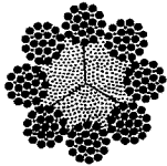
8 x 25 filler wire Type W 8 Strands, 25 Wires per Strand, 1/2 in. and larger
