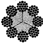
8 x 19 Warrington 8 Strands, 19 Wires per Strand, 7/16 in. and smaller
