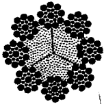
8 x 19 Seale 8 Strands, 19 Wires per Strand
