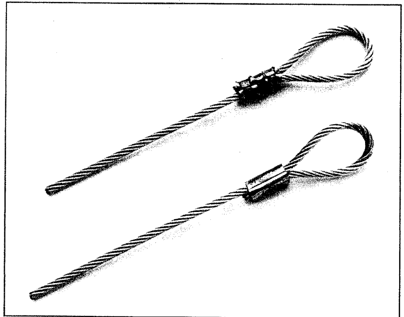
The picture above is a swaged 1/8" copper sleeve. The top assembly is swaged onto the cable.
